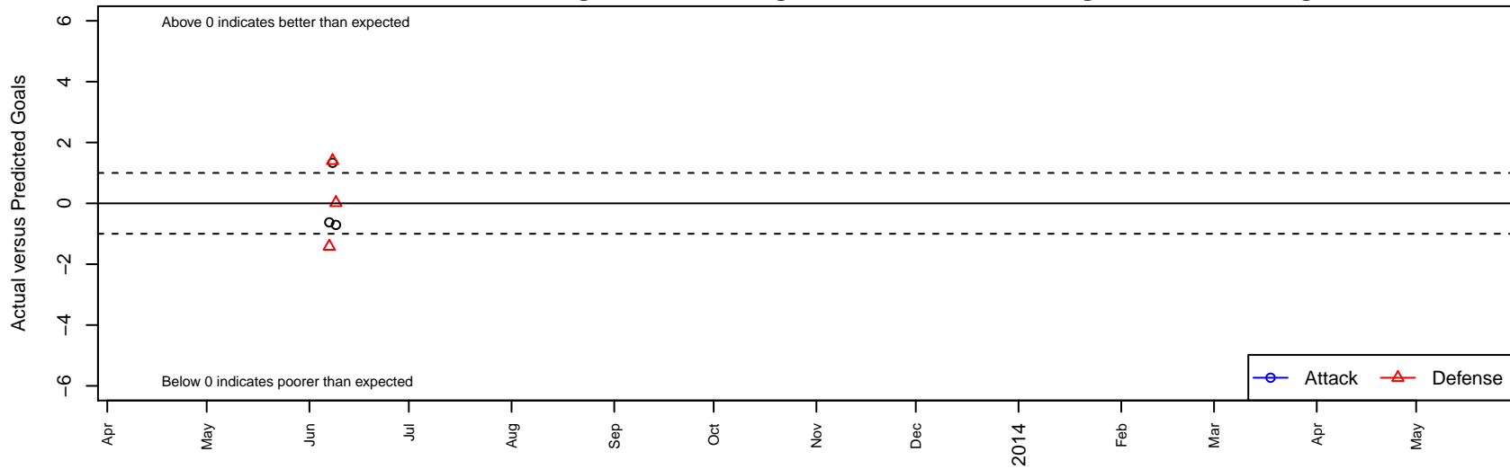
3 Rivers Wilson B97 Dots are actual minus expected GF (blue circles) and GA (red triangles). Blue line is smoothed change in attack strength. Red is smoothed change in defense strength.
